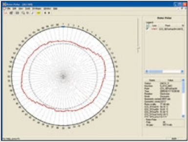
Air Gap - Rotor shape
