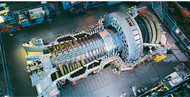
Alstom’s GT13E2 heavy duty gas turbine
